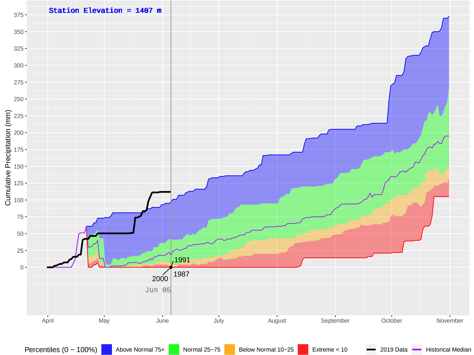
THYNNNE (279) : Historical (1977–2018), Current (2019) Daily Cumulative Precipitation
