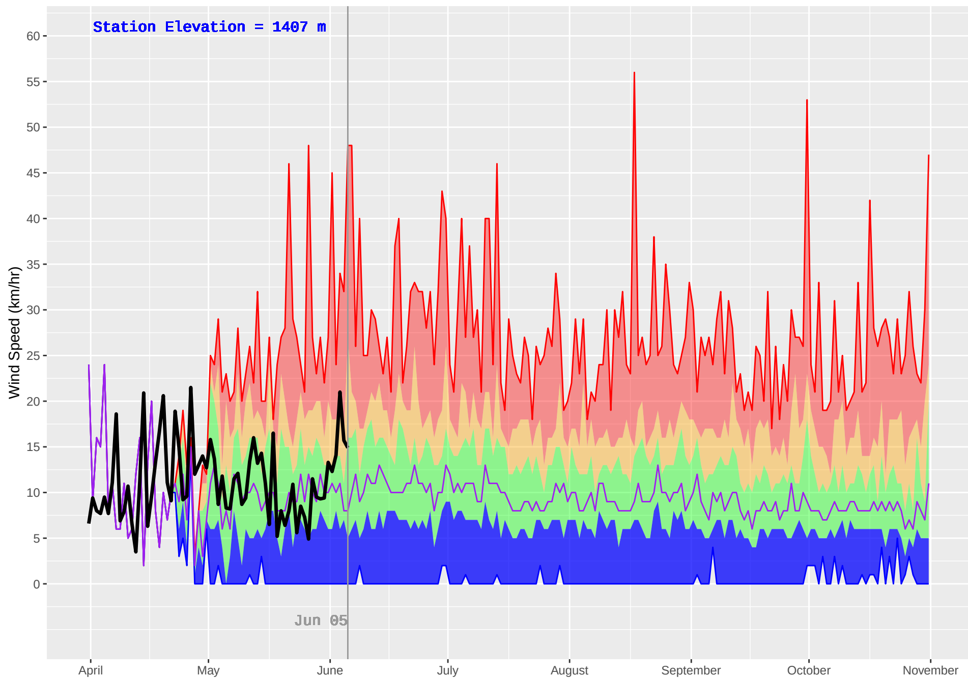
THYNNE (279) : Historical (1977–2018) and Current (2019) Daily Wind Speed
