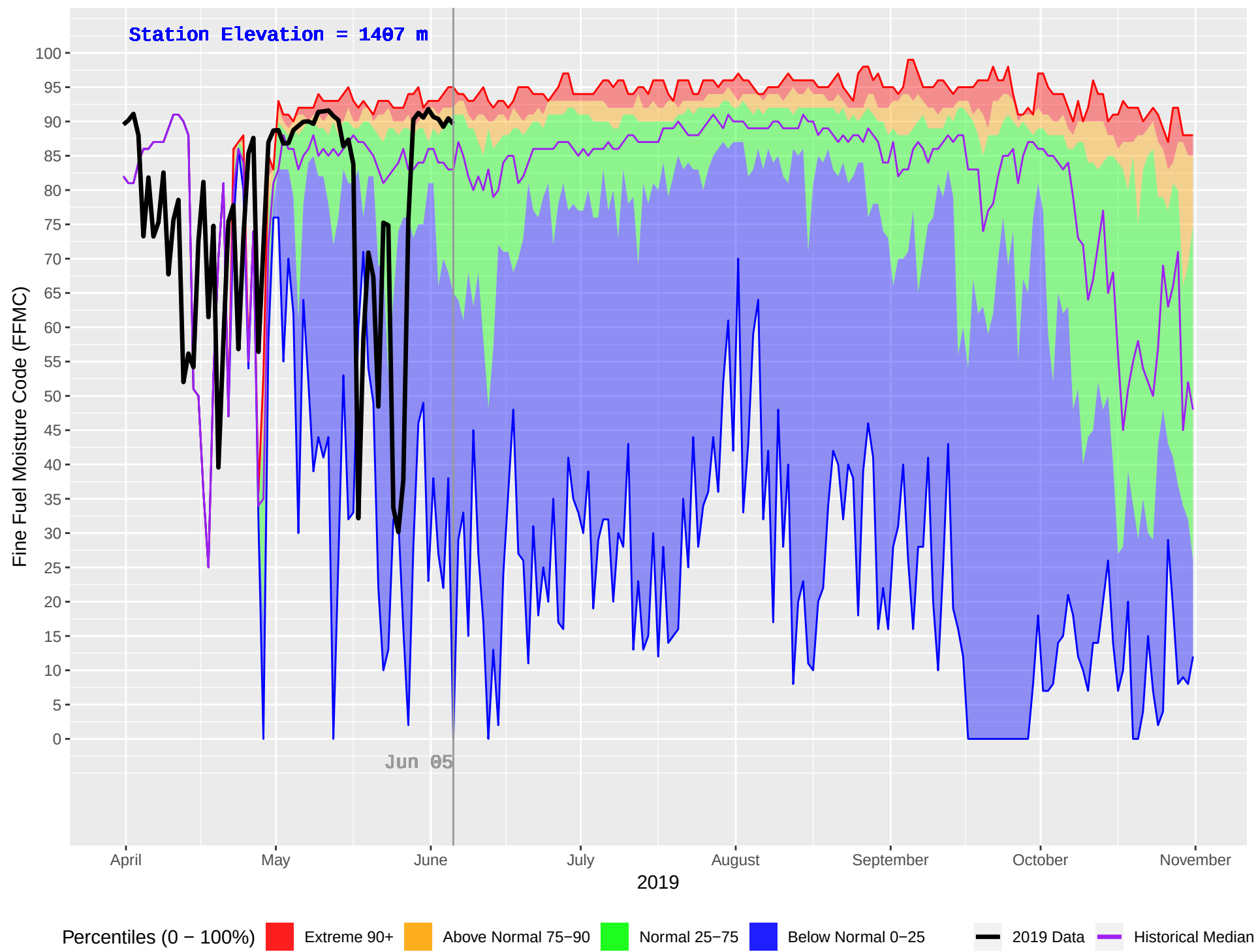
THYNNE (279) : Historical (1977–2018) and Current (2019) Daily Fine Fuel Moisture Code (FFMC)
