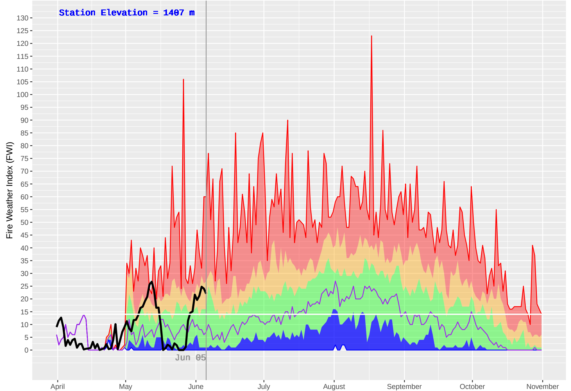
THYNNE (279) : Historical (1977–2018) and Current (2019) Daily Fire Weather Index (FWI)
