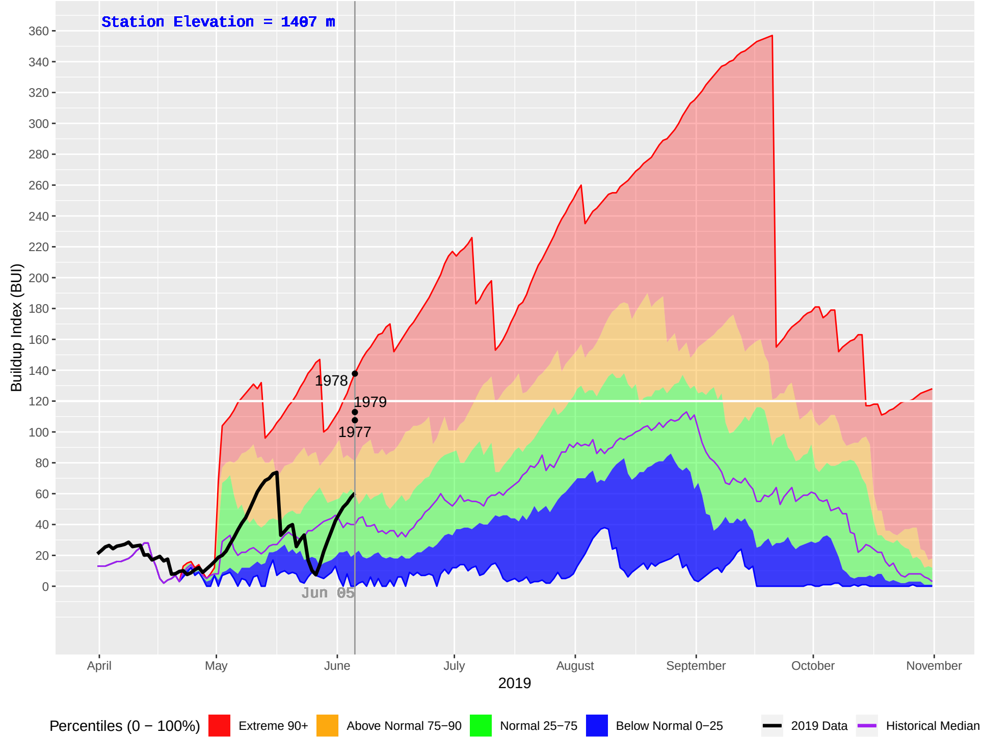
THYNNE (279) : Historical (1977–2018), Current (2019) Daily Buildup Index (BUI)
